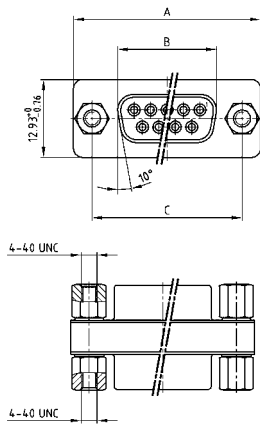
Variation socket to socket
