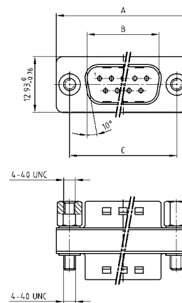
Variation plug to plug
